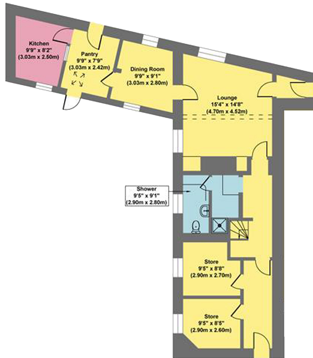
Ground Floor
